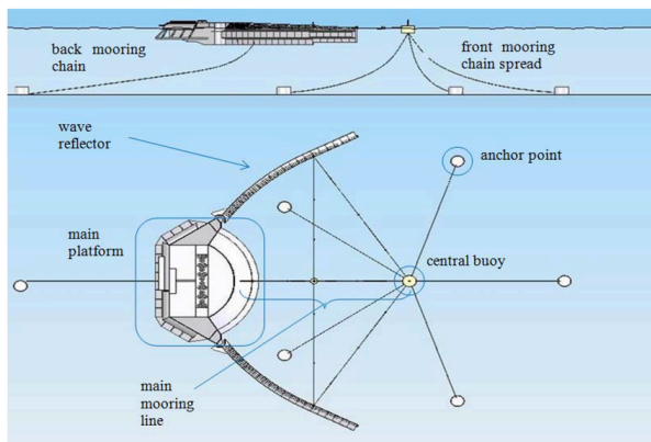
Wave Dragon mooring diagram
